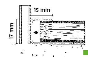
FN fit-fix Nr. 6 6-7 mm
