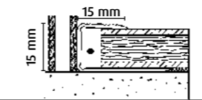
FN fit-fix Nr. 14 14-15 mm
