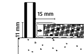
FN fit-fix Nr. 3 10-11 mm
