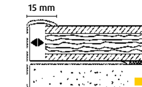
FN fit-fix Nr. 5 13-15 mm
