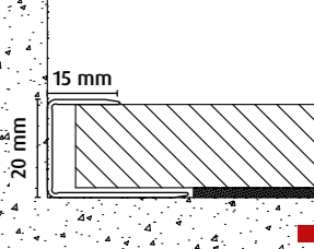
FN fit-fix Nr. 15 17-18 mm
