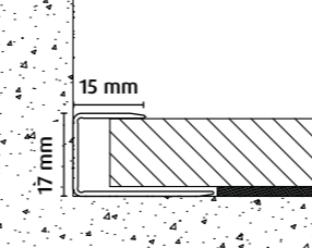
FN fit-fix Nr. 14 14-15 mm
