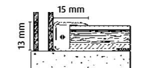
FN fit-fix Nr. 7 12-13 mm
